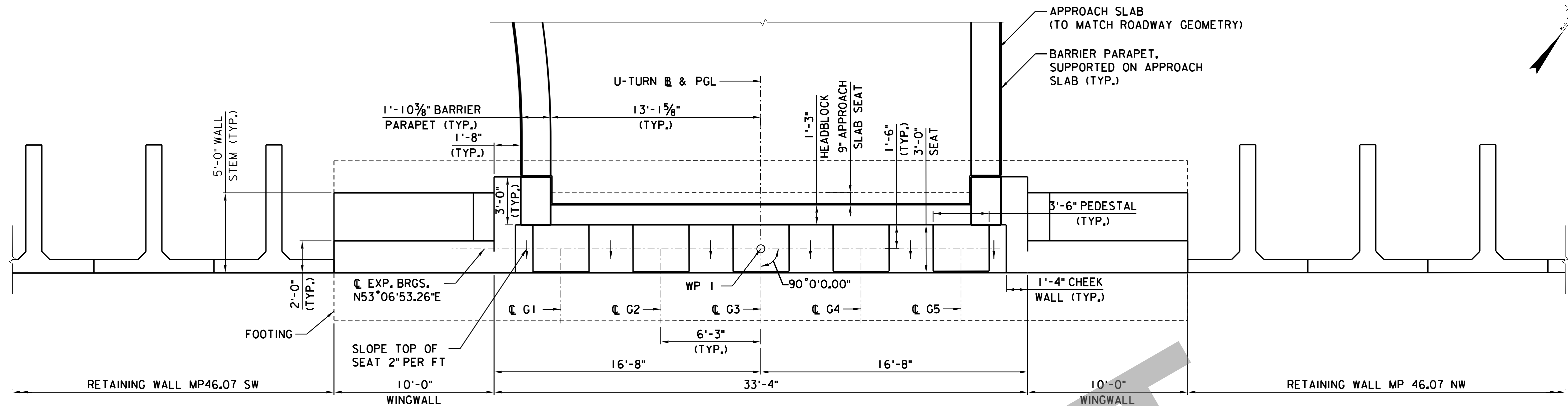
PLAN 1/4" = 1'-0"
