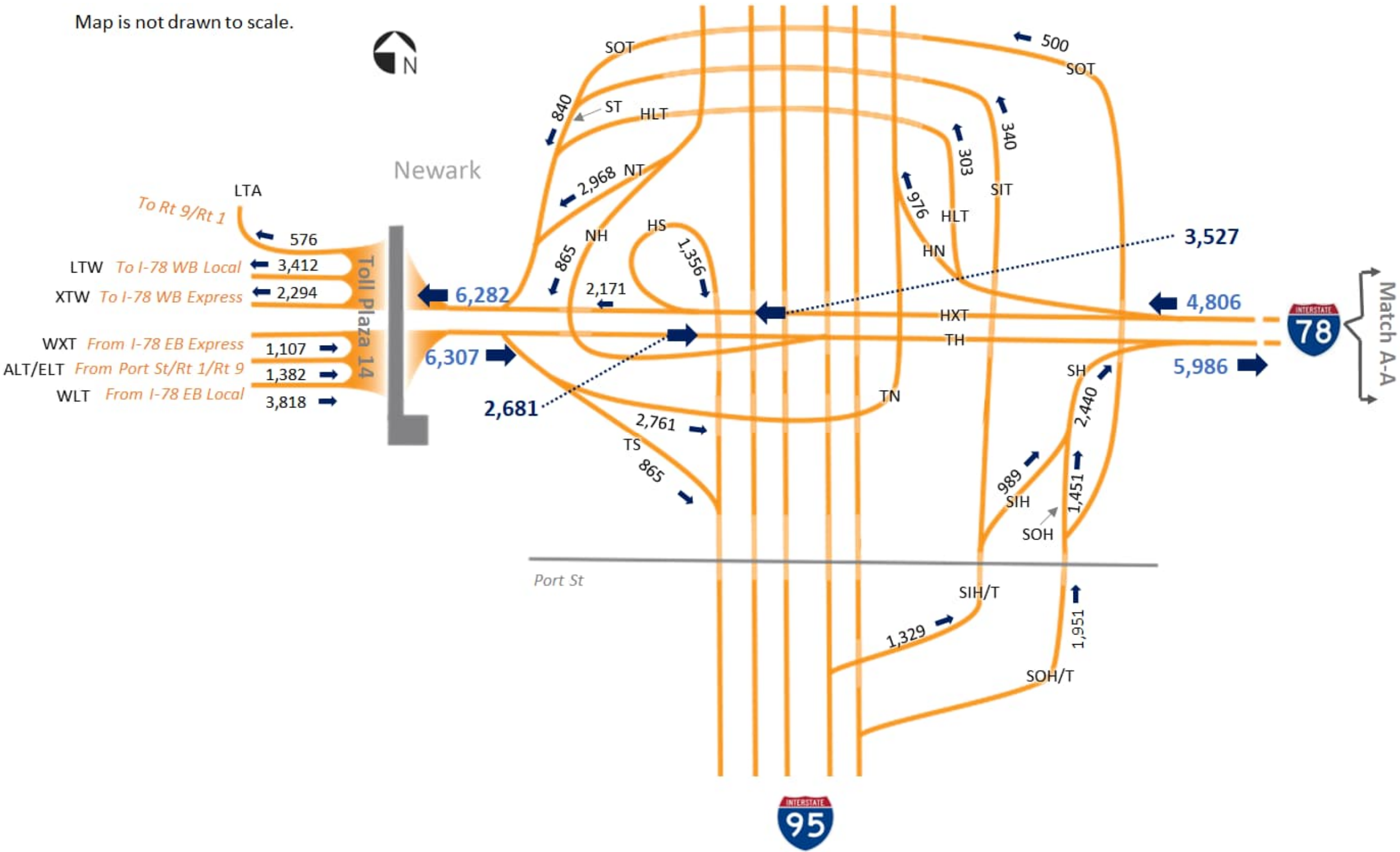
2050 Build AM Peak Hour Volumes (Interchange 14)
