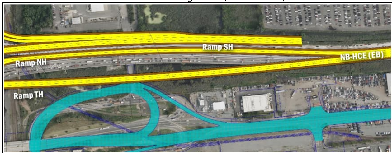
Figure 10-8 – Ramp TH/Ramp NH/Ramp SH Junction (Interchange 14) Alternative 4 Alignment (Eastern Limit)
