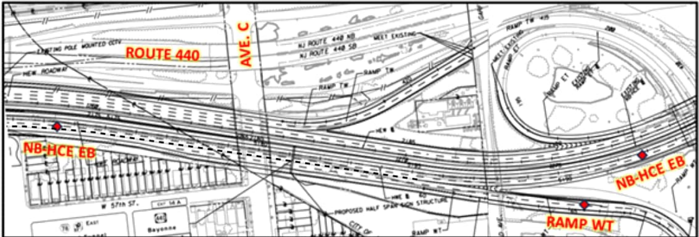
Figure 10-14 – NB-HCE Eastbound at Ramp WT (Interchange 14A) Proposed Geometry – Alternative 1 (IPA)
