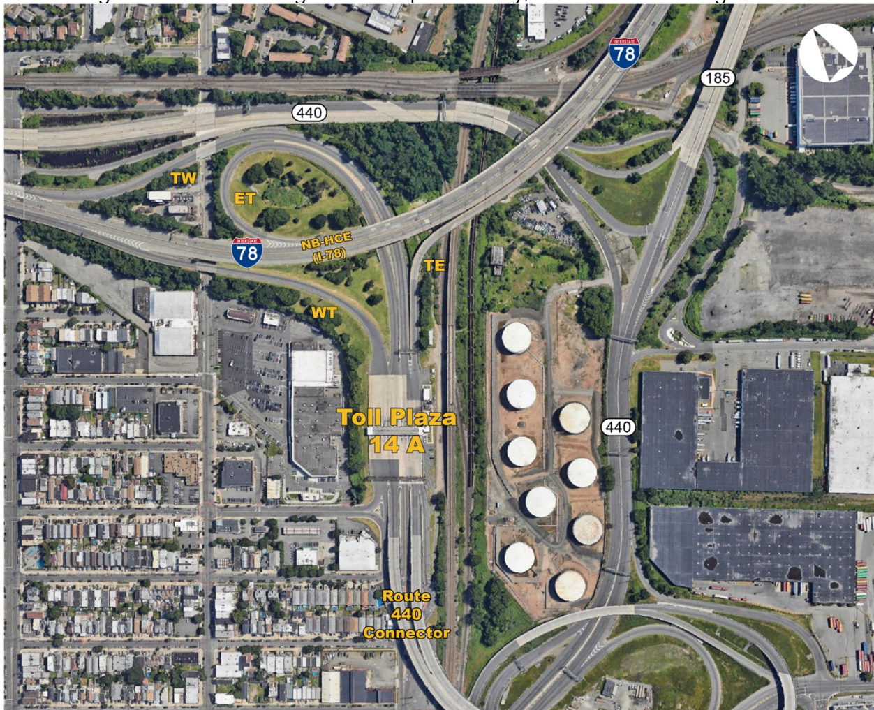
Figure C-7 – Interchange 14A Ramp Geometry, Locations and Designations
