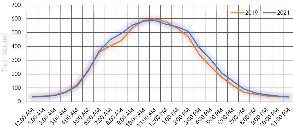
Figure 7-3 – Weekday Truck Activity by Time of Day (2019 and 2021) NB-HCE (Both Directions) Between Interchange 14 and Interchange 14A
