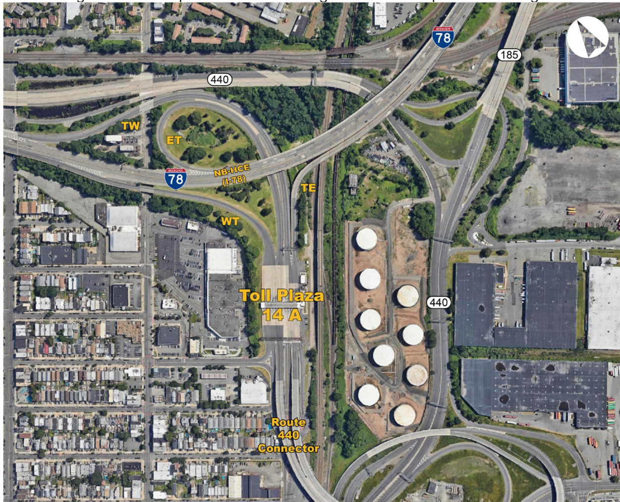
Figure 9-2 - Ramp Locations and Designations at Turnpike Interchange 14A
