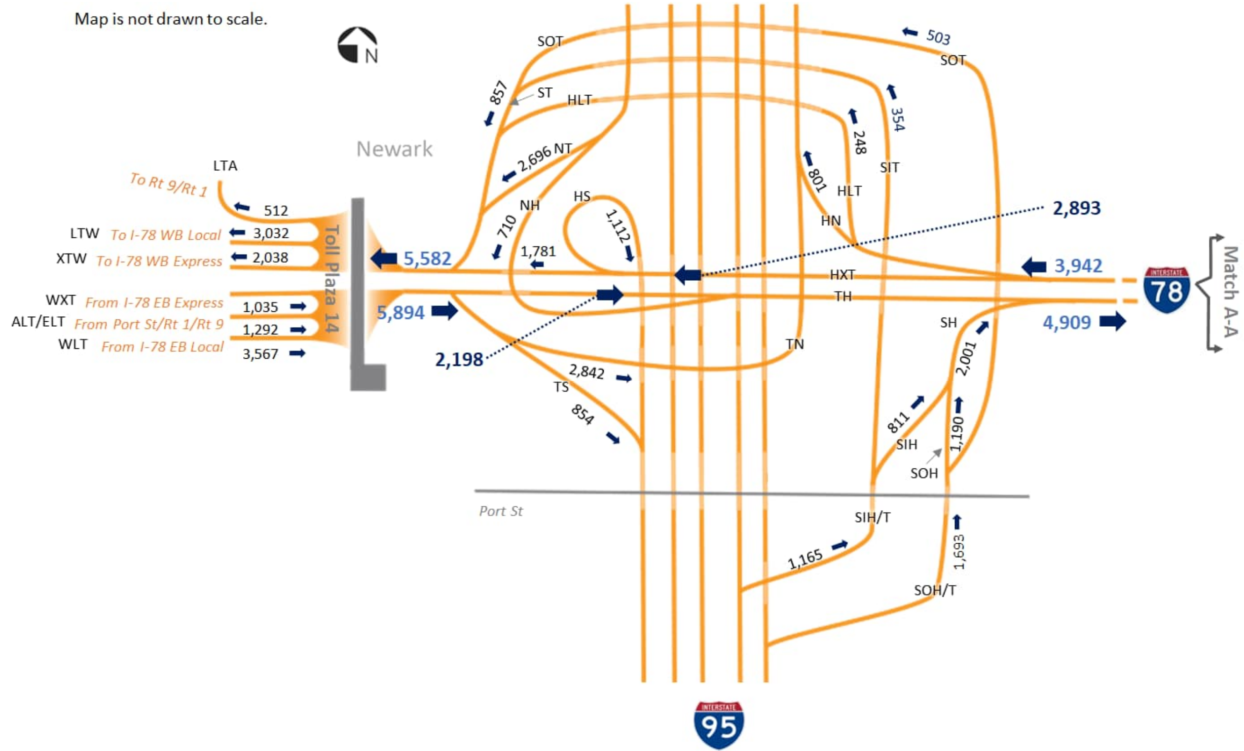
2050 No-Build AM Peak Hour Volumes (Interchange 14)
