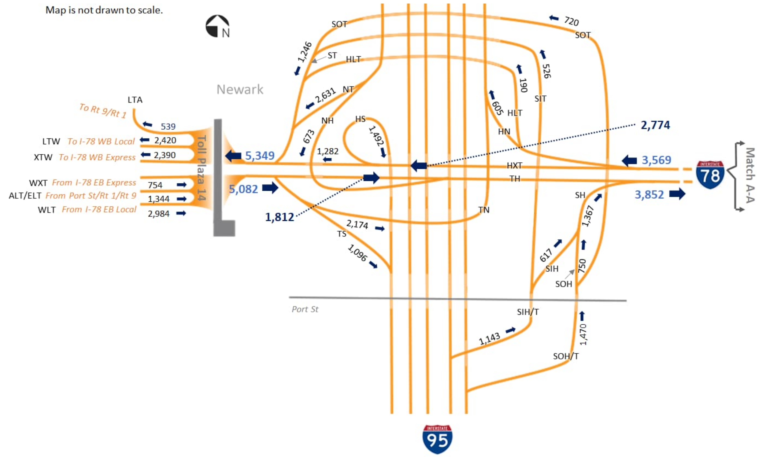
2021 PM Peak Hour Volumes (Interchange 14)
