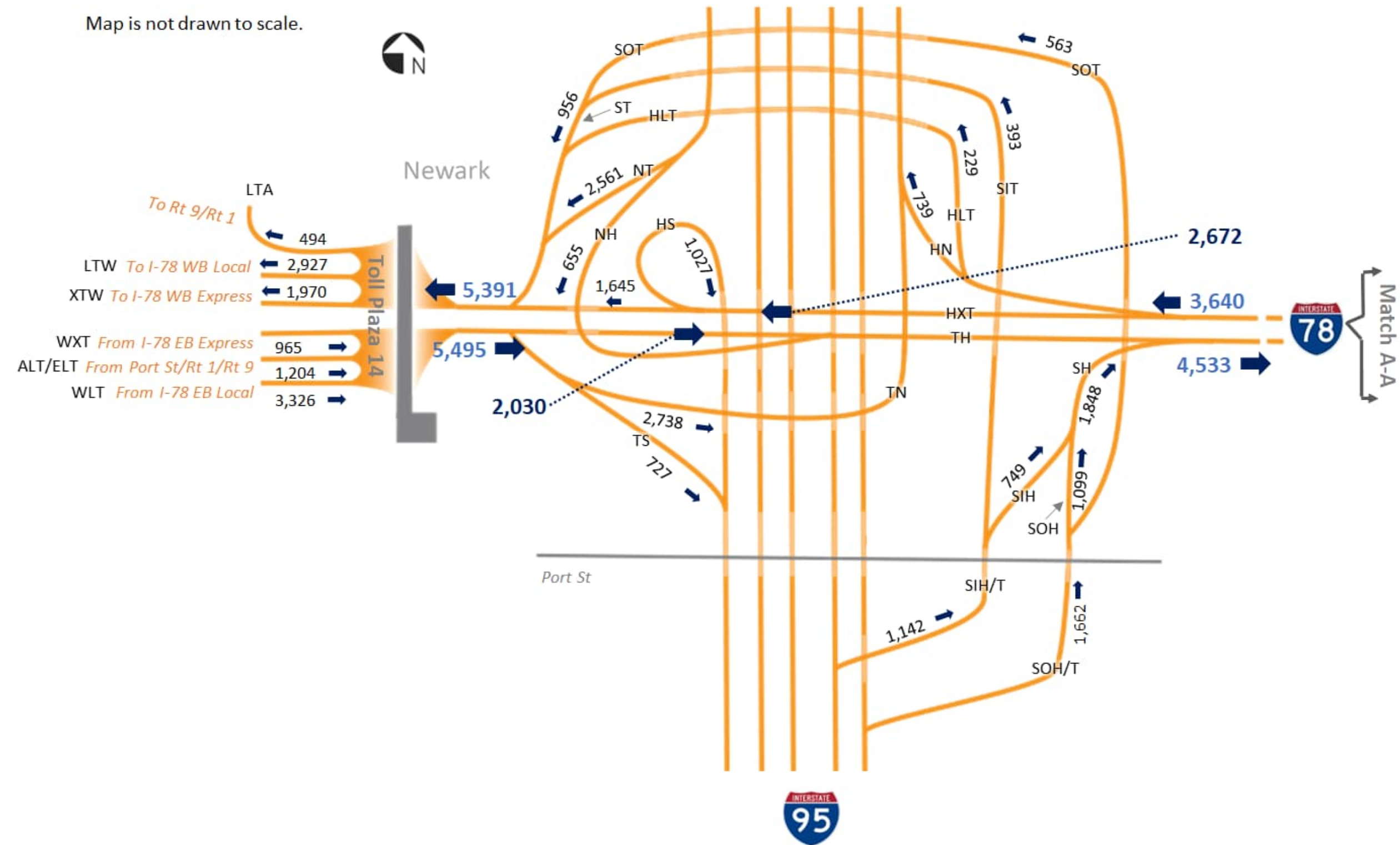
Hour Volumes (Interchange 14)
