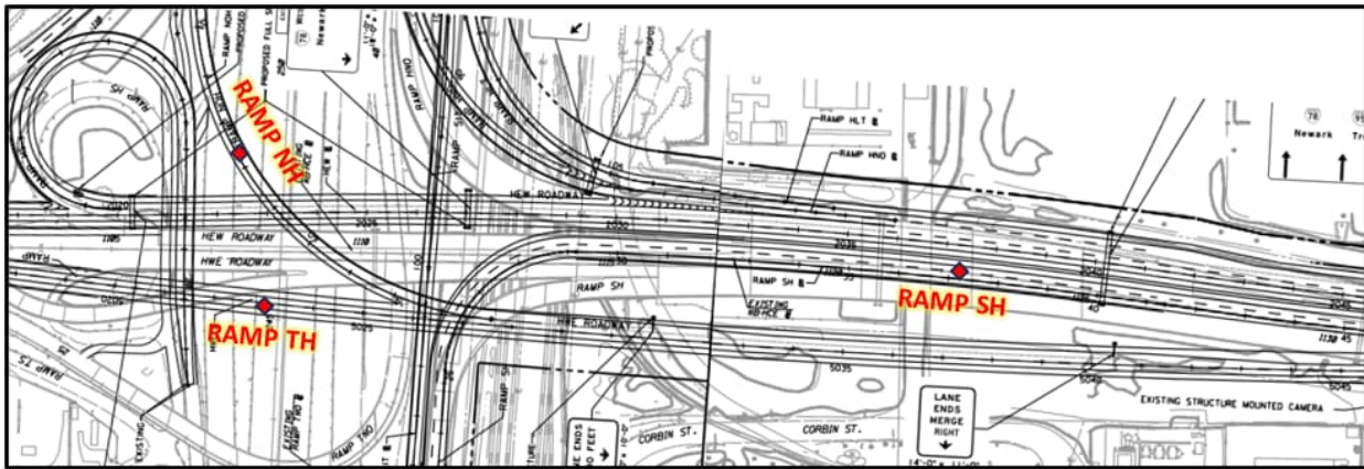
Figure 10-10 – Ramp TH/Ramp NH/Ramp SH Junction (Interchange 14) Alternative 5 Alignment (Eastern Limit)
