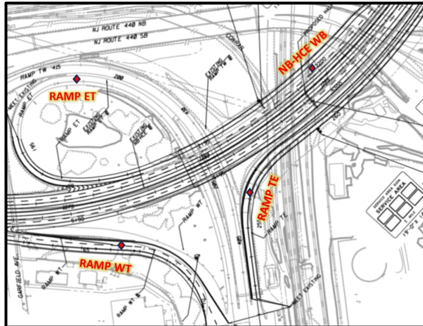
Proposed Geometry (IPA) – Eastern Segment
