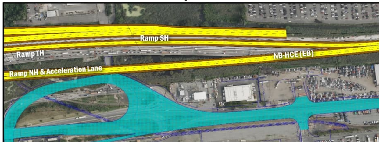
Figure 10-6– Ramp TH/Ramp NH/Ramp SH Junction (Interchange 14) Alternative 3 Alignment (Eastern Limit)
