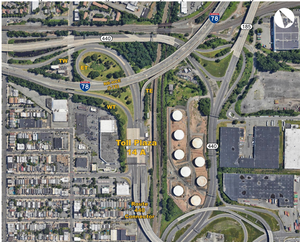
Figure 3-3 – Interchange 14A Geometry, Ramp Locations and Designations
