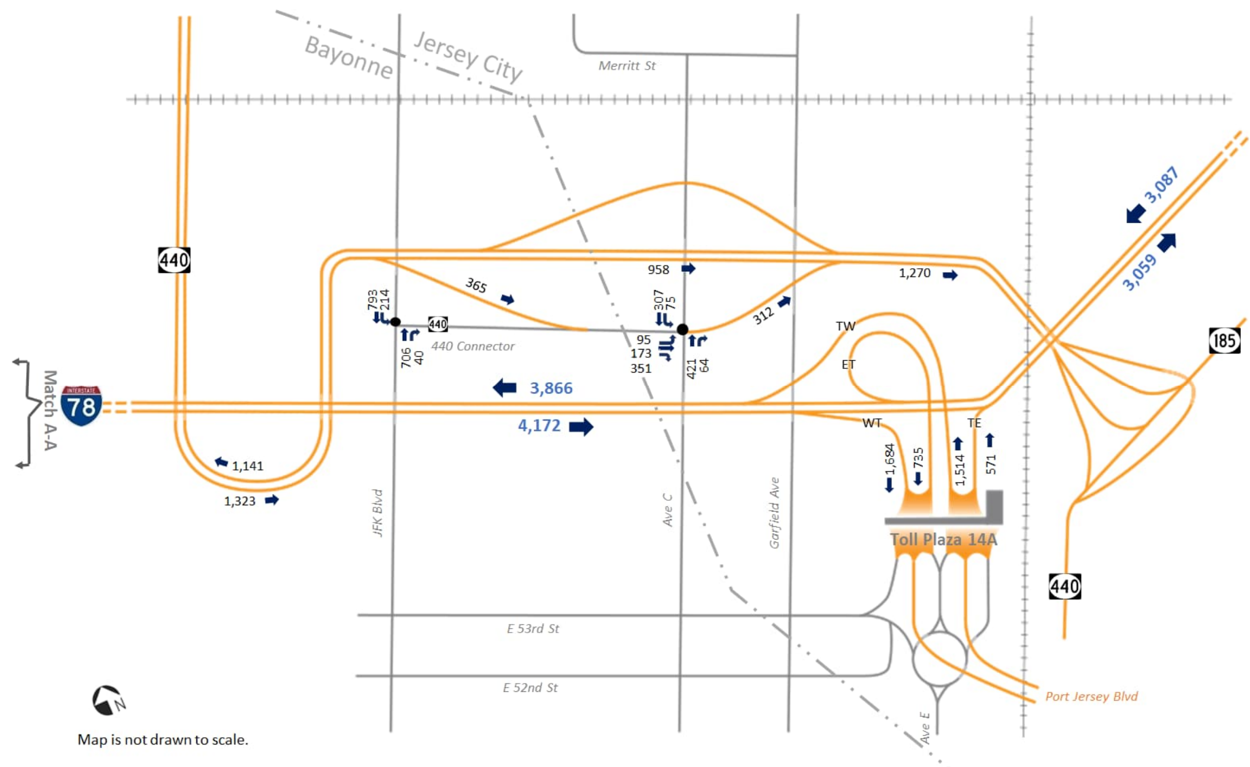
2050 No-Build PM Peak Hour Volumes (Interchange 14A)
