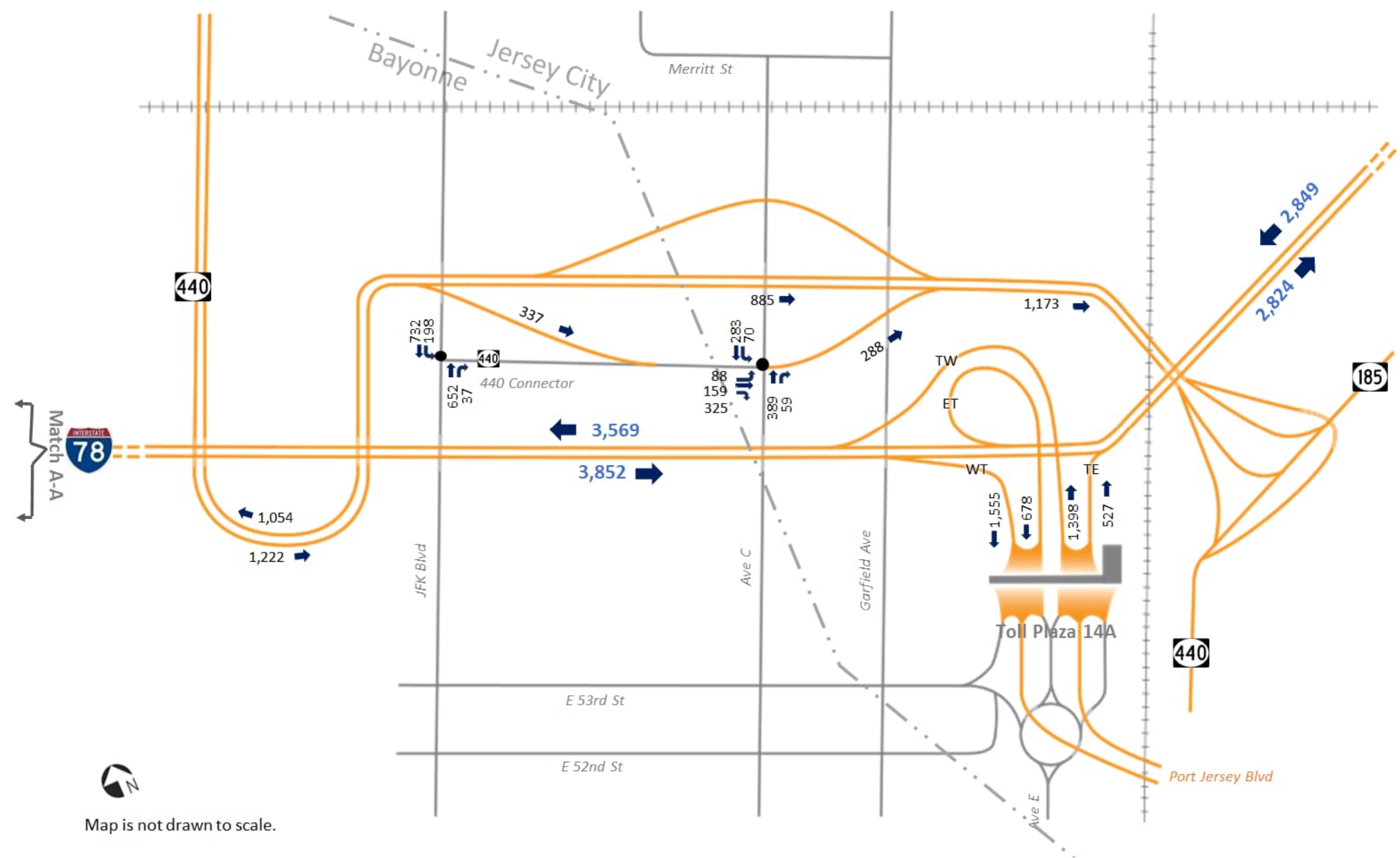
2021 PM Peak Hour Volumes (Interchange 14A)
