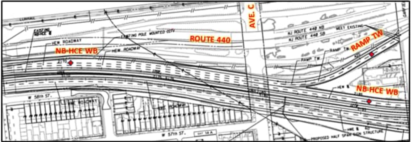
Proposed Geometry (IPA) – Western Segment
