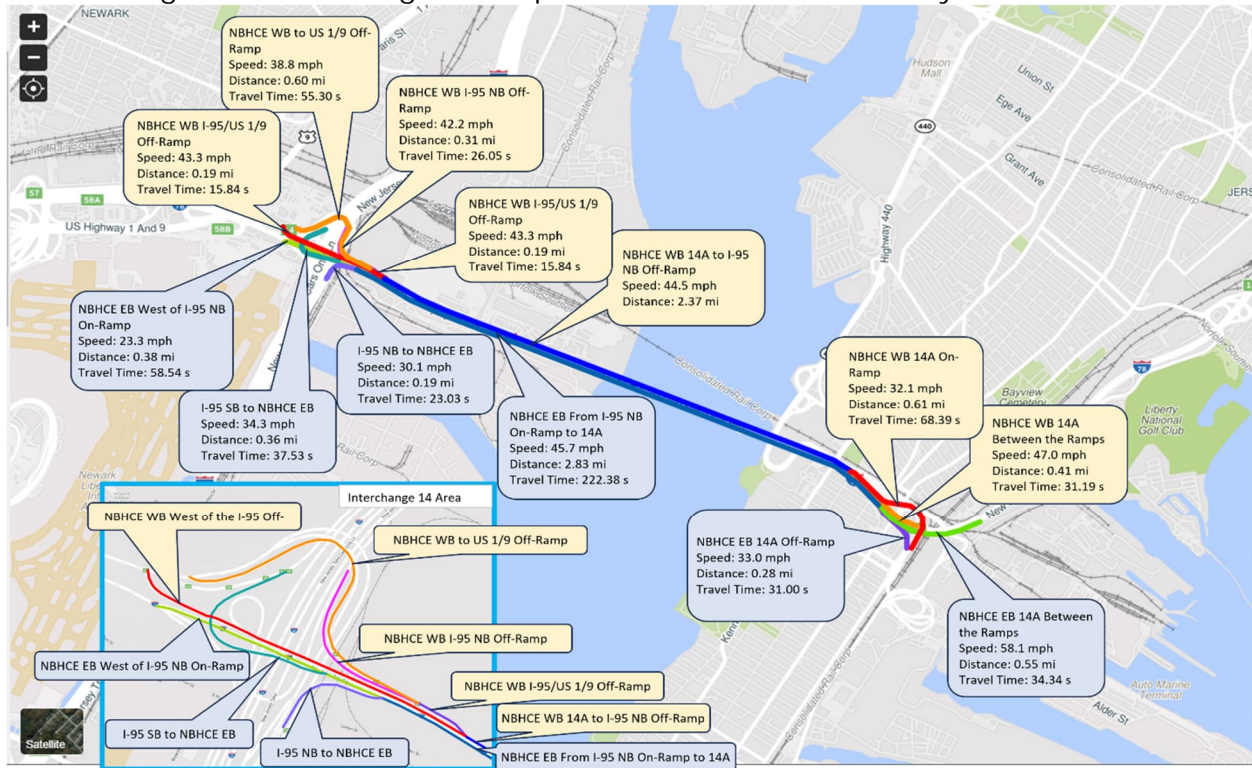
Figure 8-2 – Existing Travel Speeds from RITIS for Weekday PM Peak Hour
