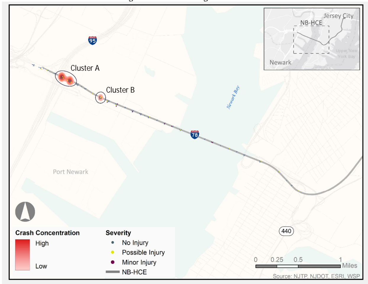
Figure C-1 - Crash Clusters in Project Limits Interchange 14 to Interchange 14A – Eastbound
