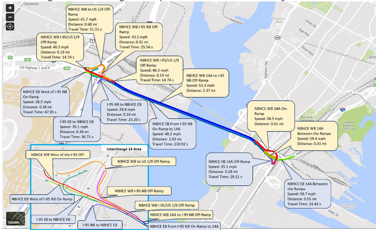
Figure 8-1 – Existing Travel Speeds from RITIS for Weekday AM Peak Hour
