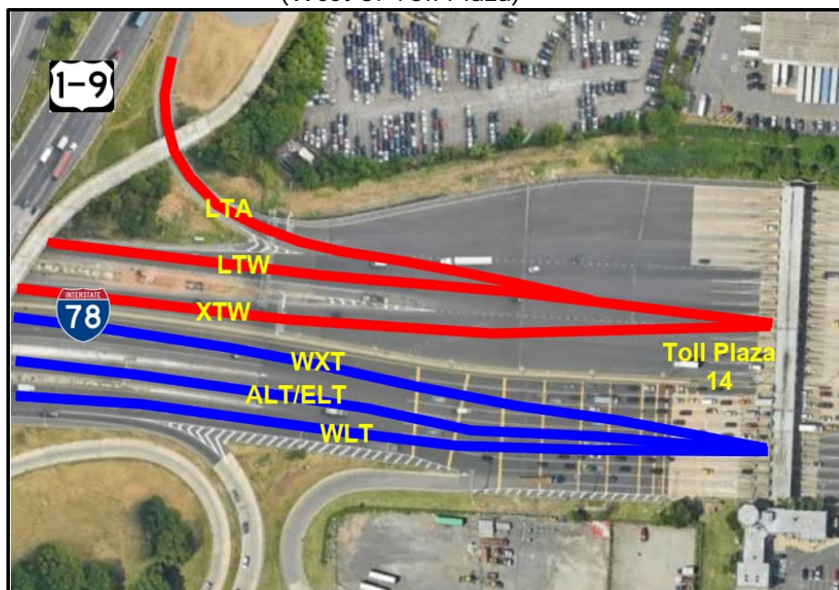
Figure 3-1 - Interchange 14 Toll Plaza Ramp/Roadway Locations and Designations (West of Toll Plaza)
