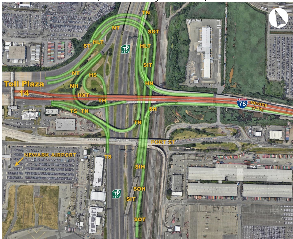
Figure 3-2 – Interchange 14 Geometry, Ramp Locations and Designations (East of Interchange 14 Toll Plaza)
