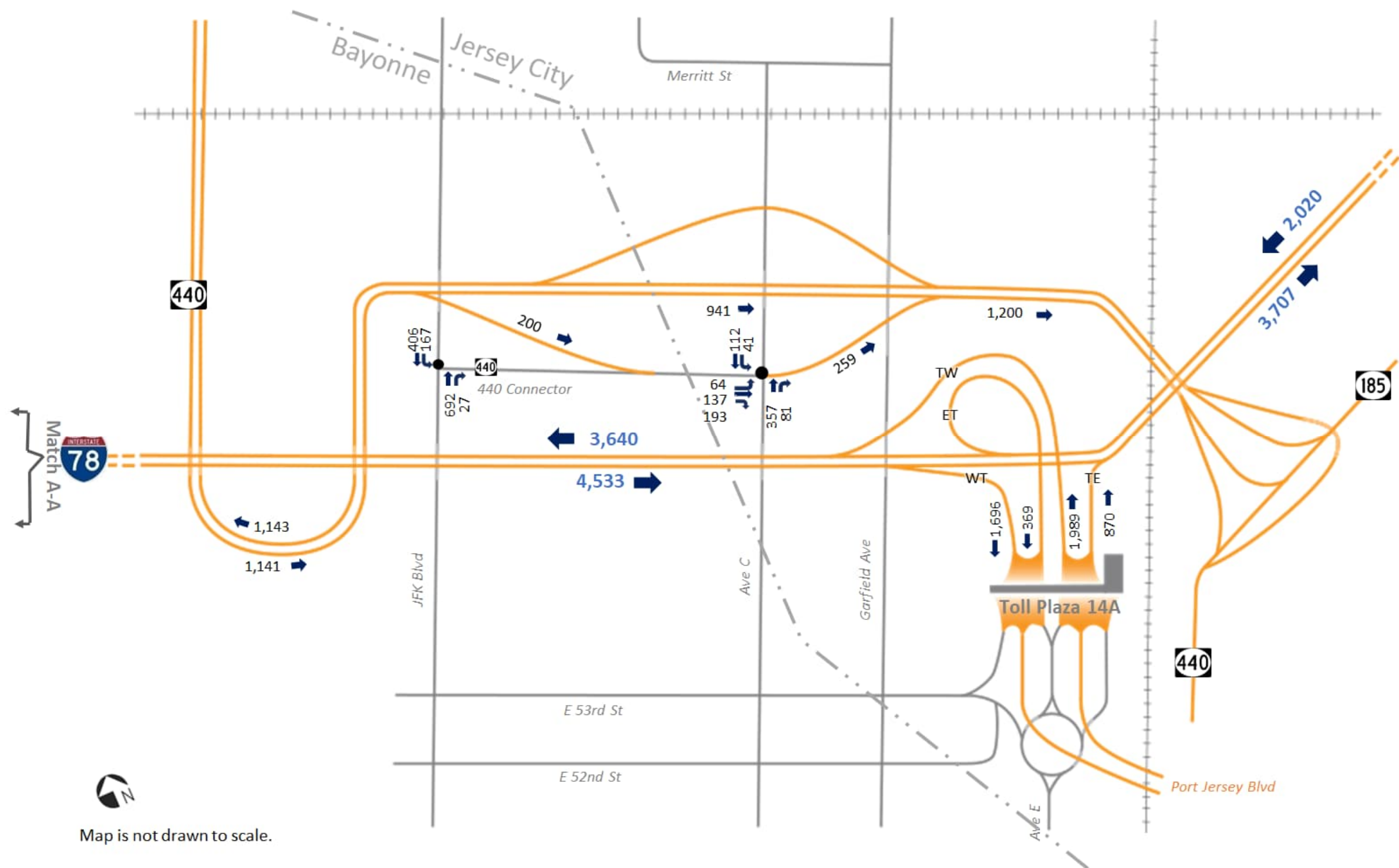
2021 AM Peak Hour Volumes (Interchange 14A)
