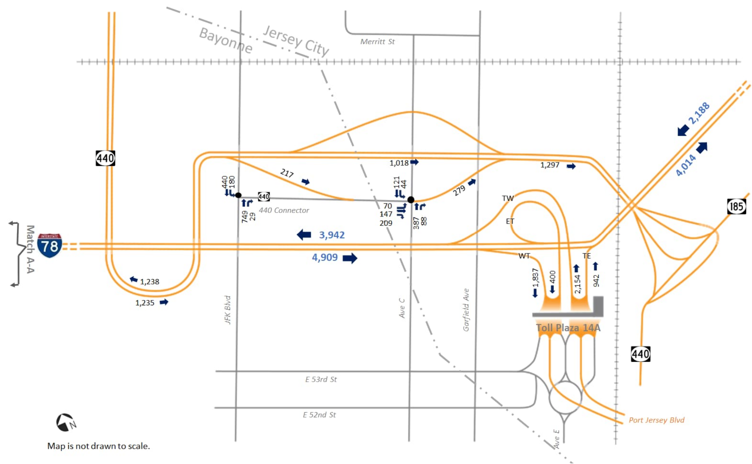
2050 No-Build AM Peak Hour Volumes (Interchange 14A)
