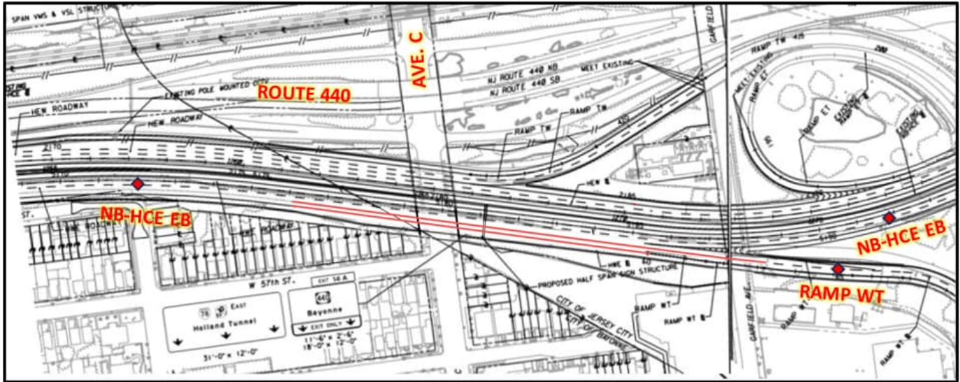
Figure 10-15 – NB-HCE Eastbound at Ramp WT (Interchange 14A) Proposed Geometry – Alternative 2 (Option Lane)
