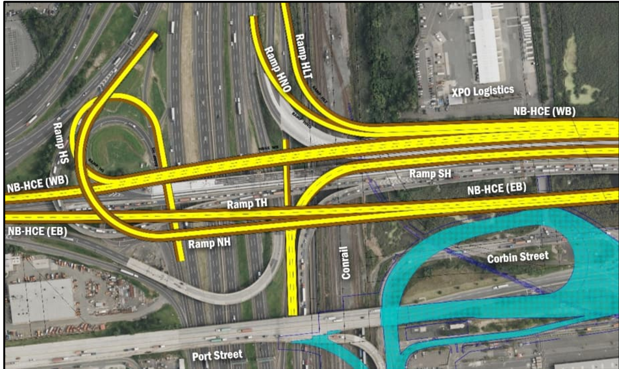
Figure 10-5 – Ramp TH/Ramp NH/Ramp SH Junction (Interchange 14) Alternative 3 Alignment (Western Limit)
