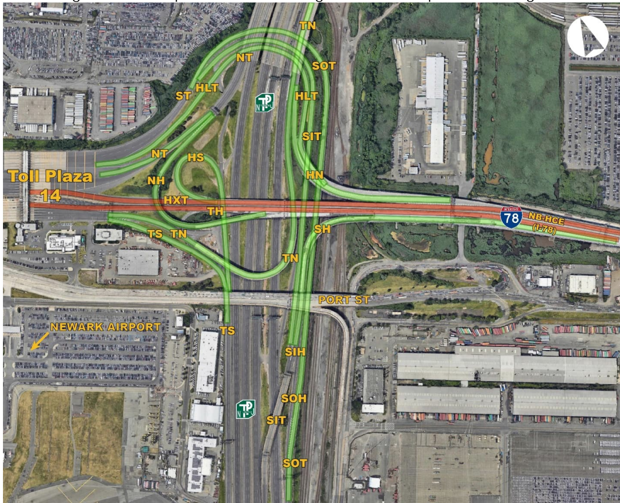
Figure 9-1 - Ramp Locations and Designations at Turnpike Interchange 14
