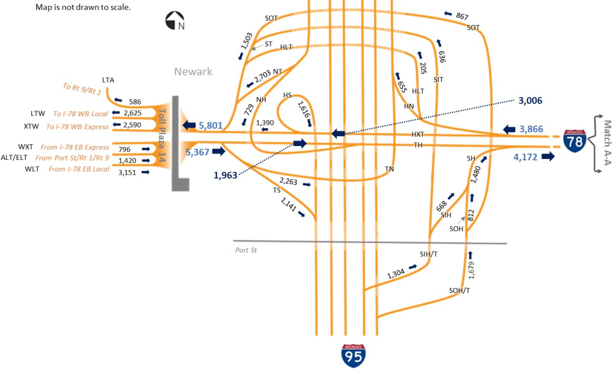
2050 No-Build PM Peak Hour Volumes (Interchange 14)
