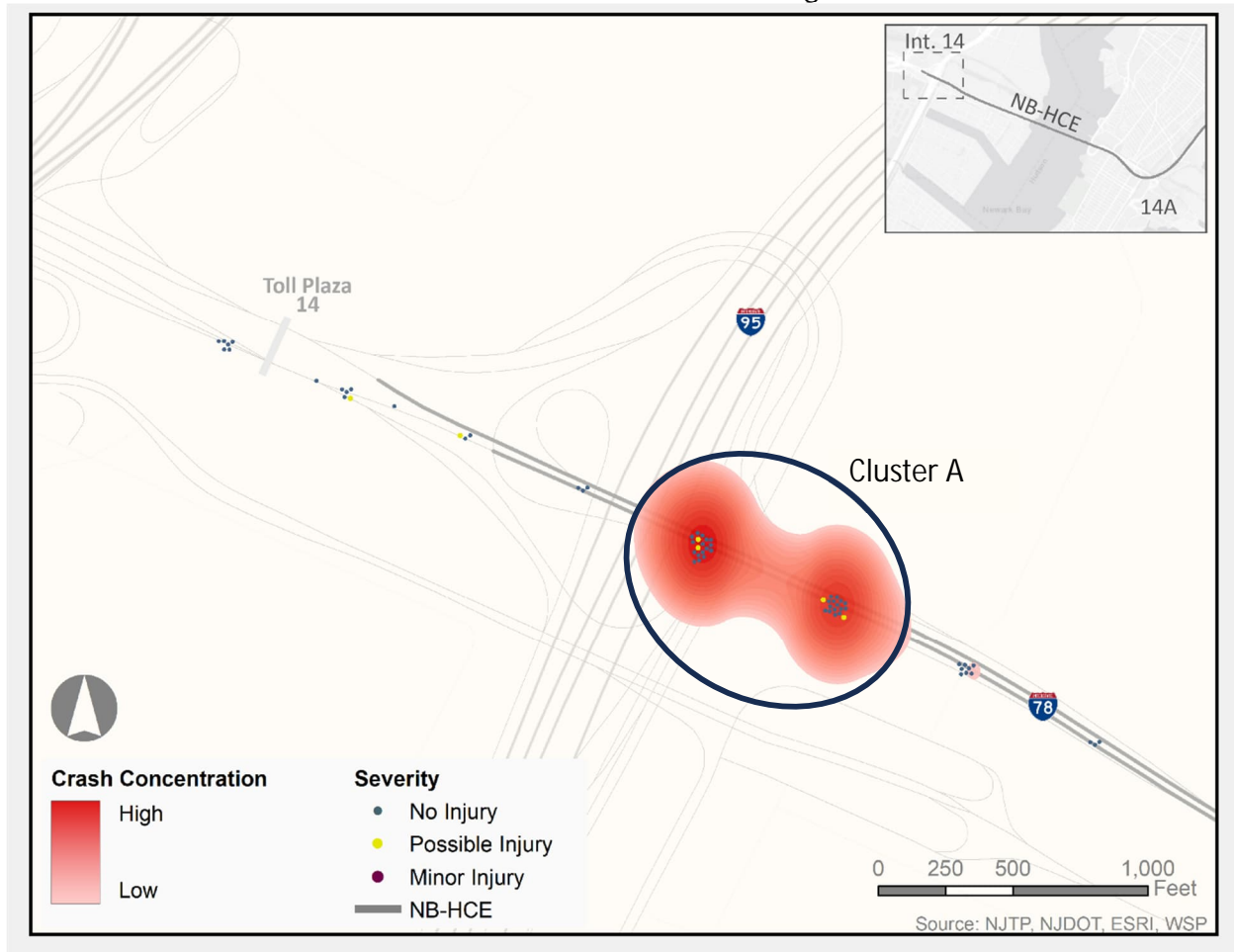
Figure C-3 - Crash Clusters in Project Limits NB-HCE Eastbound at Interchange 14
