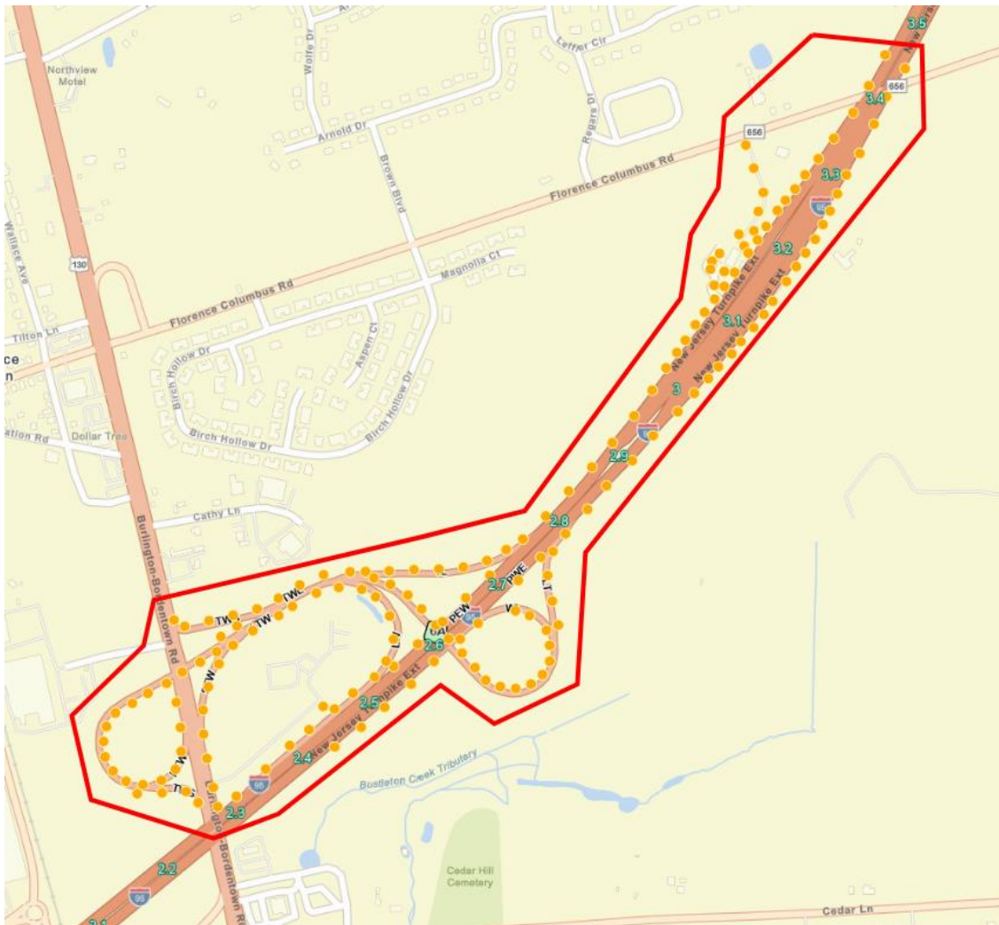
New Jersey Turnpike Interchange 6/6A MP 2.3 to MP 3.5
