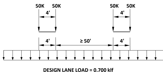
Figure 3.2.1-2 – TP-16 Design Load Models
