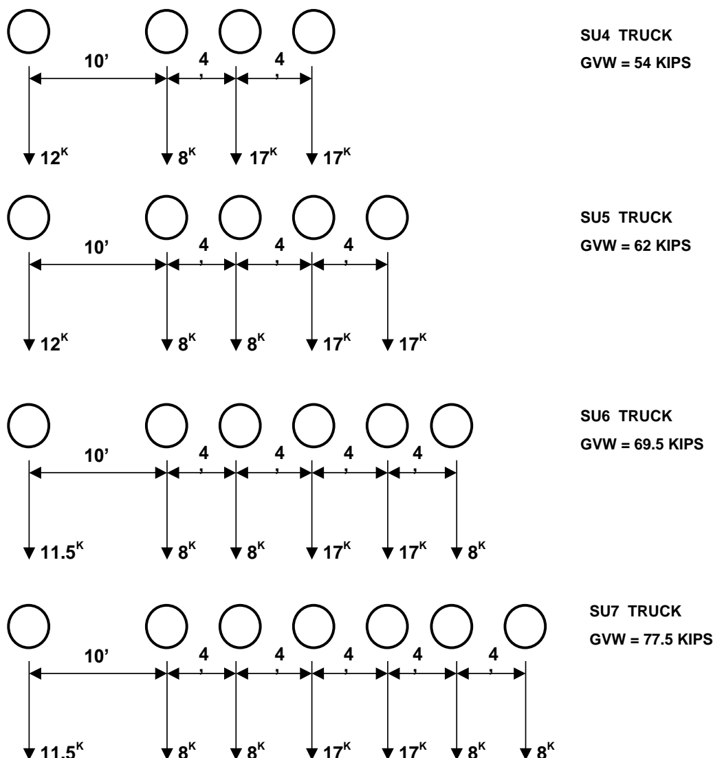
Figure 3.2.3 - AASHTO Legal Loads for SHV
