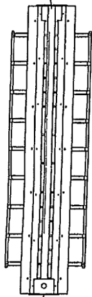
PLAN VIEW OF 10' 4 CONTACT TREADLE FRAME WITH DUAL DRAINS SCALE: 3/32"=1"
