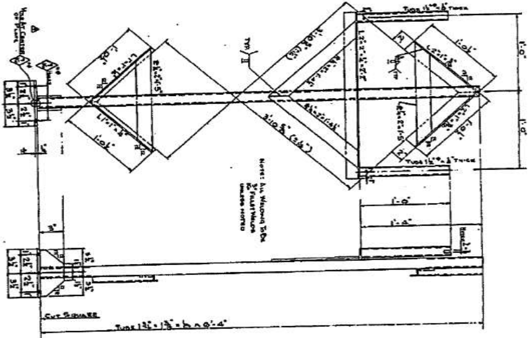
CONCRETE MEDIAN BARRIER SADDLE
