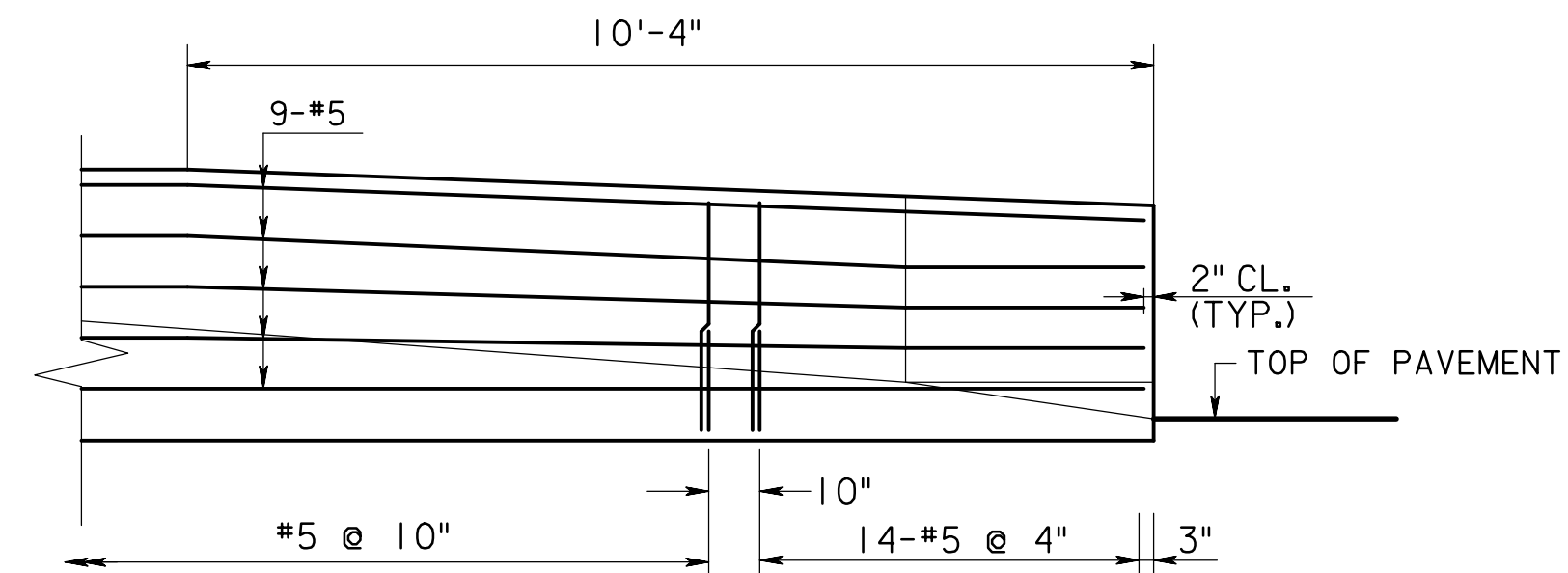
INTERIOR ELEVATION, BARRIER PARAPET (TYPE A & B CONNECTIONS) N.T.S.
