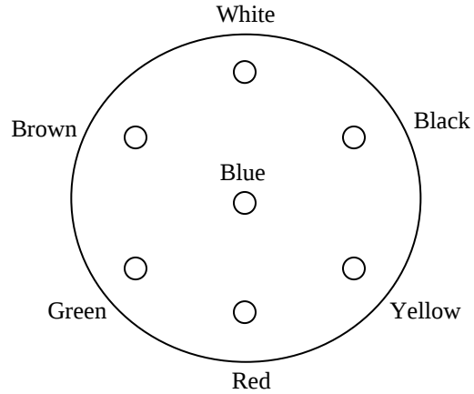
PLUG MARKINGS
