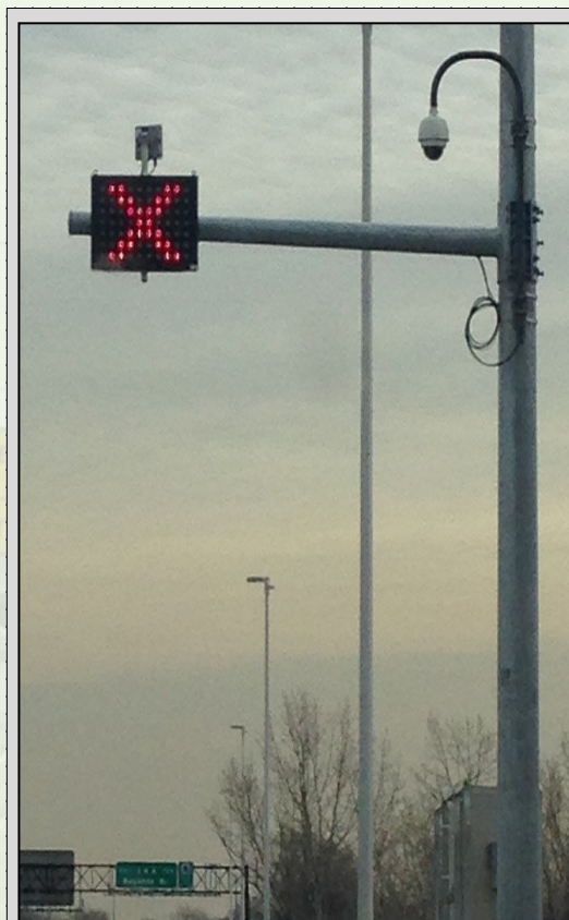
The Lane Control System on the NBHCE, which lets drivers know when the shoulder is open to traffic, will be decommissioned starting on or about May 20, 2019.
