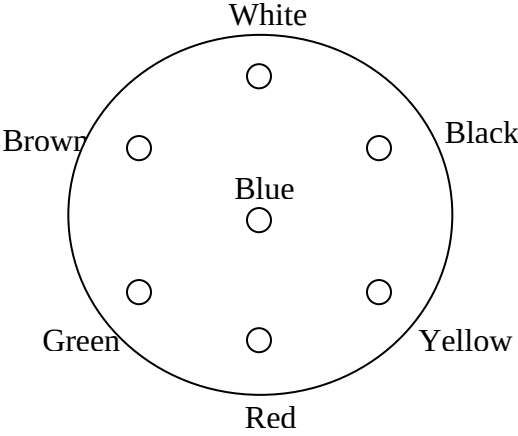
PLUG MARKINGS
