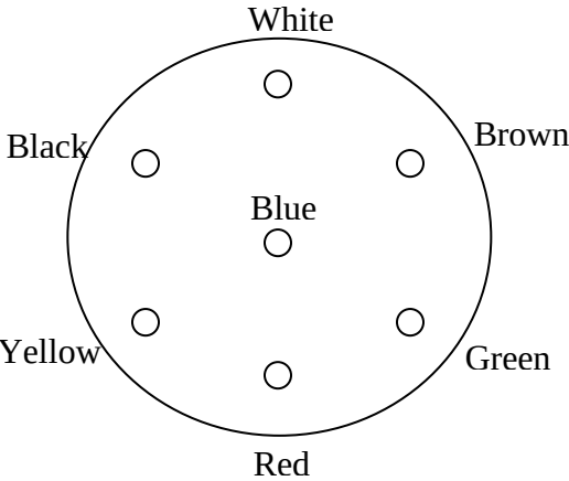
SOCKET MARKINGS
