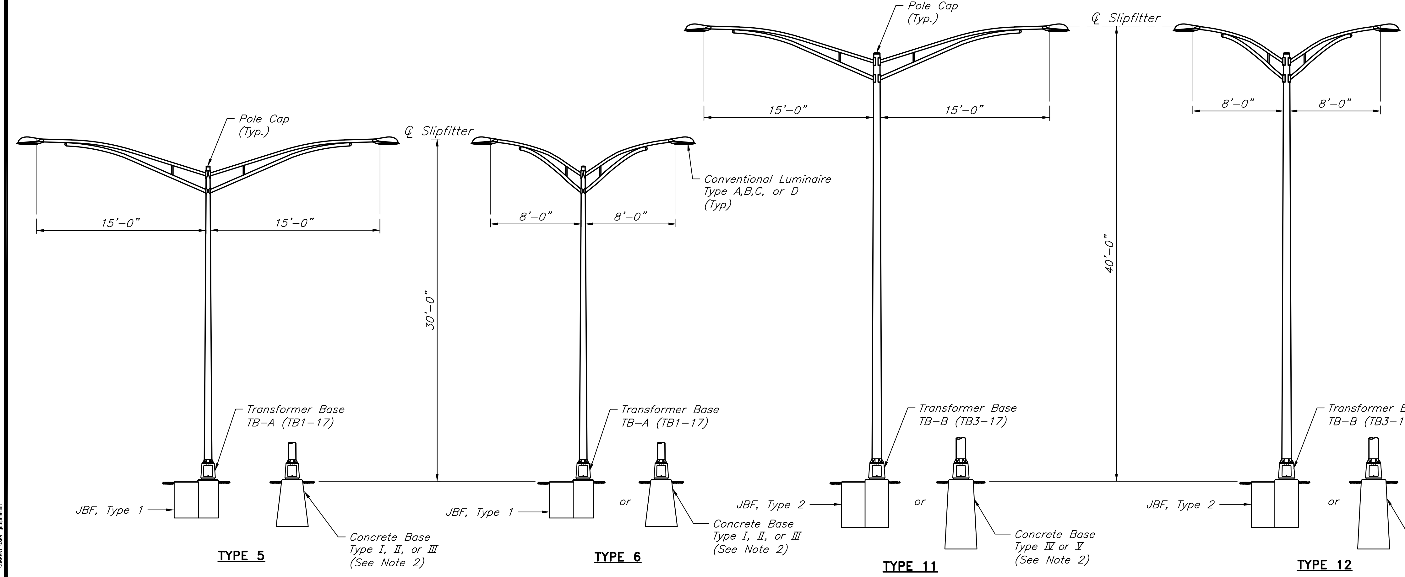
TYPICAL LIGHTING STANDARD TYPES Scale: 3/16" = 1'-0"
