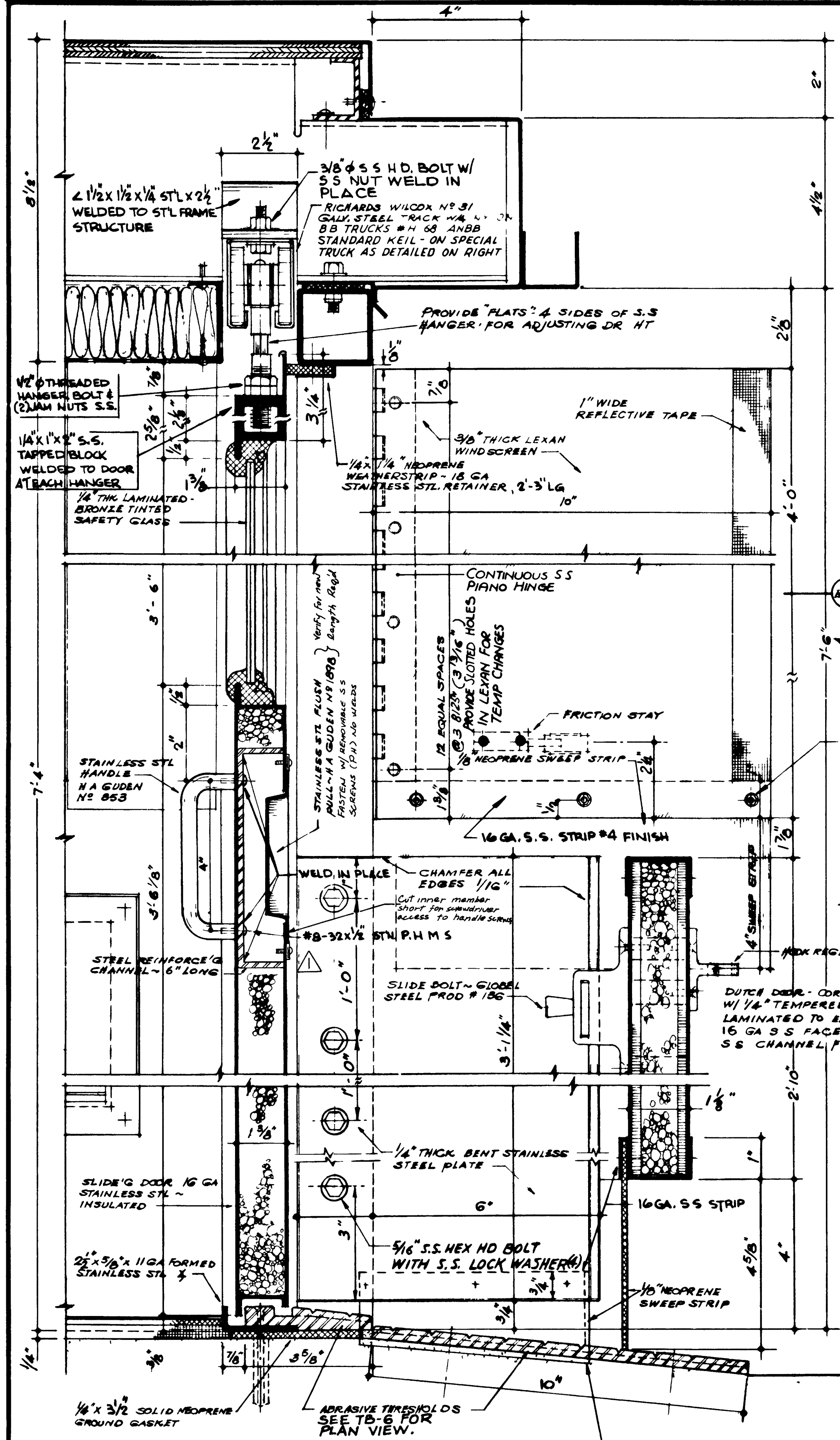
SECTION - HS 5 SCALE - HALF FULL SIZE (AT SLIDE G DOOR, DUTCH DOOR and WINDSCREEN)
