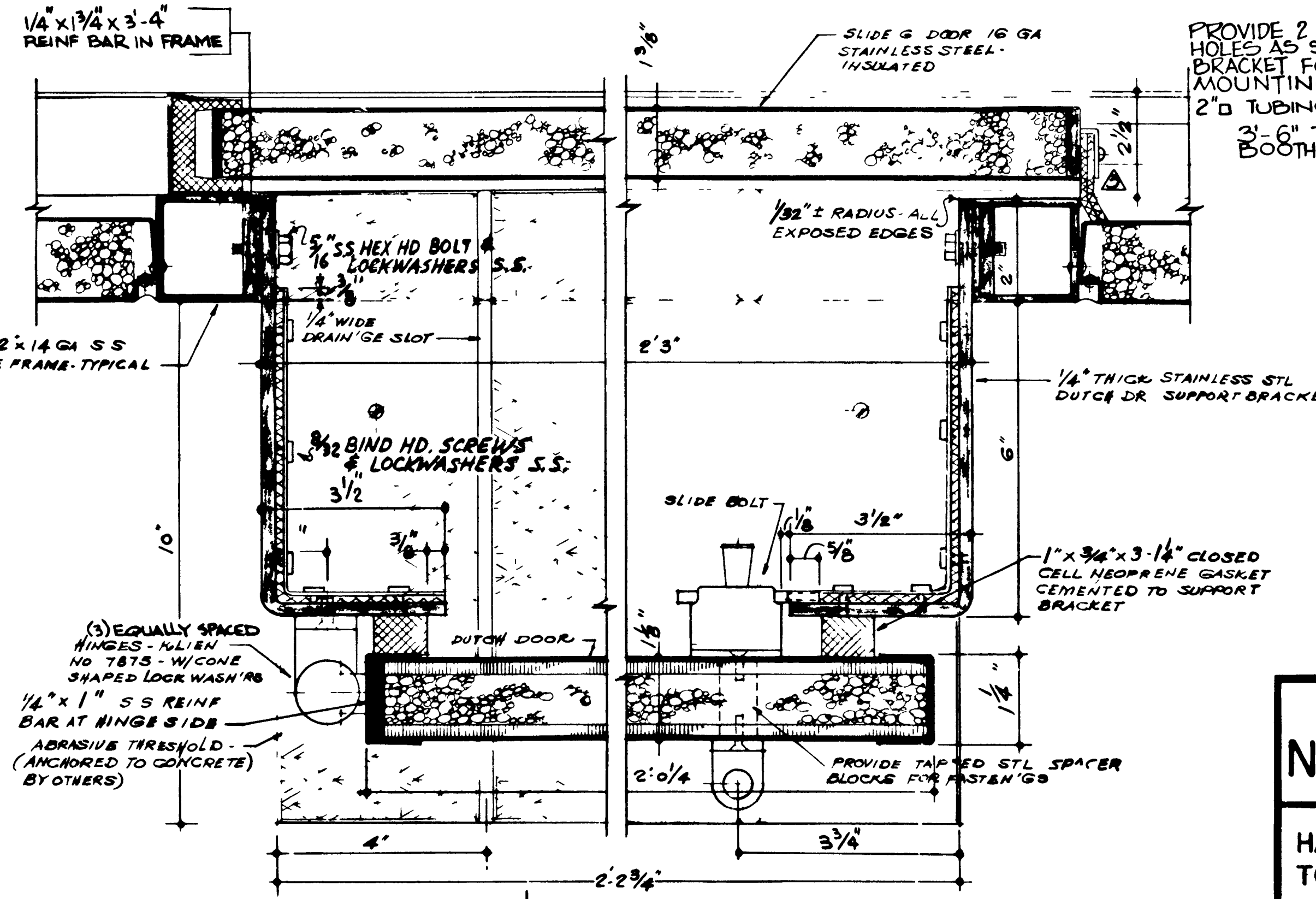
PLAN SECTION - HS 7 SCALE - HALF FULL SIZE (AT DUTCH DOOR)
