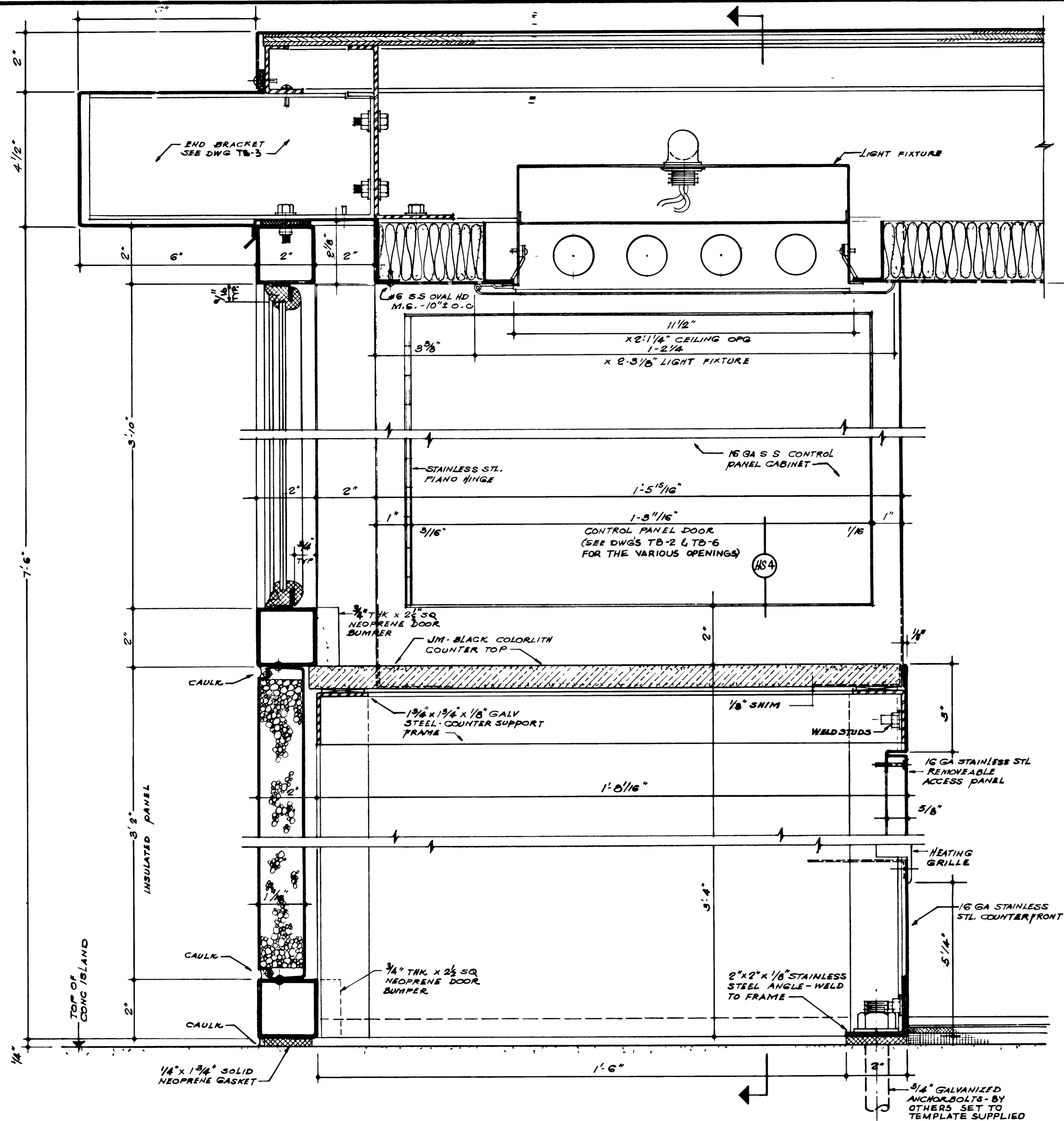
SECTION - HS-3 SCALE - HALF FULL SIZE (THRU REAR OF BOOTH)
