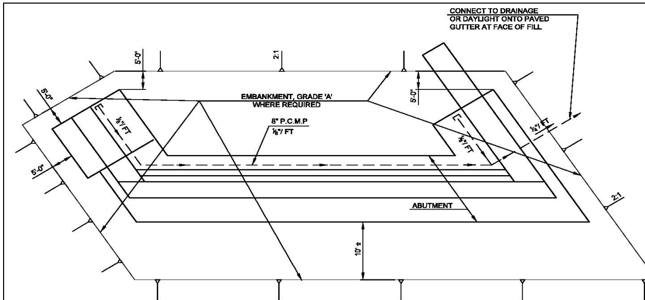
DETAIL 1 CONVENTIONAL ABUTMENT PLAN NTS
